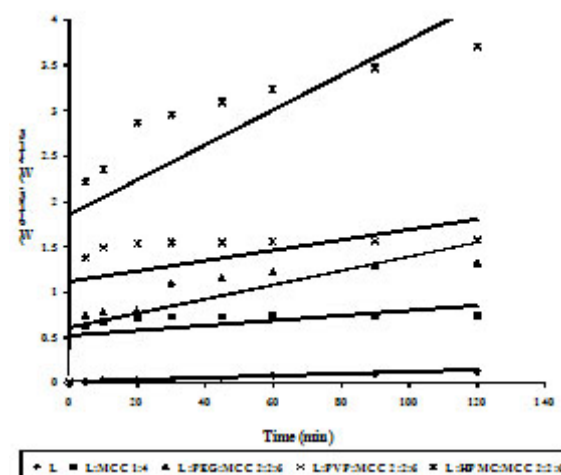
Fig. 4 : Hixson-Crowell Dissolution Plots of Lornoxicam and its Solid Dispersions
